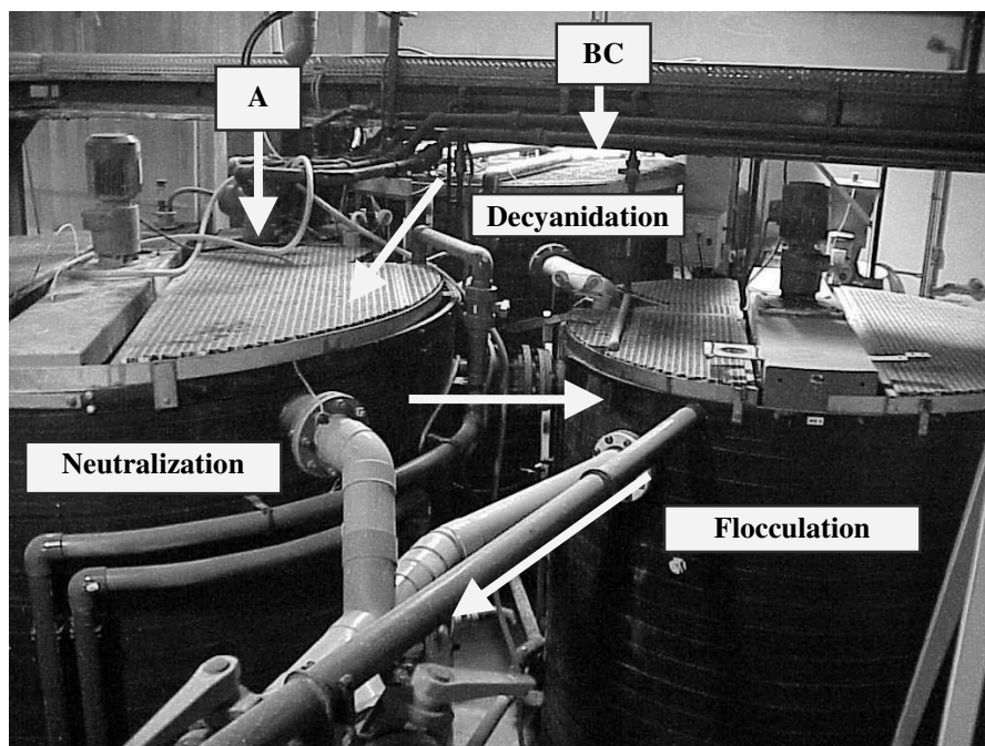
Figure 1. Picture of a part of an industrial WWDP. Arrows show effluents flow directions.
