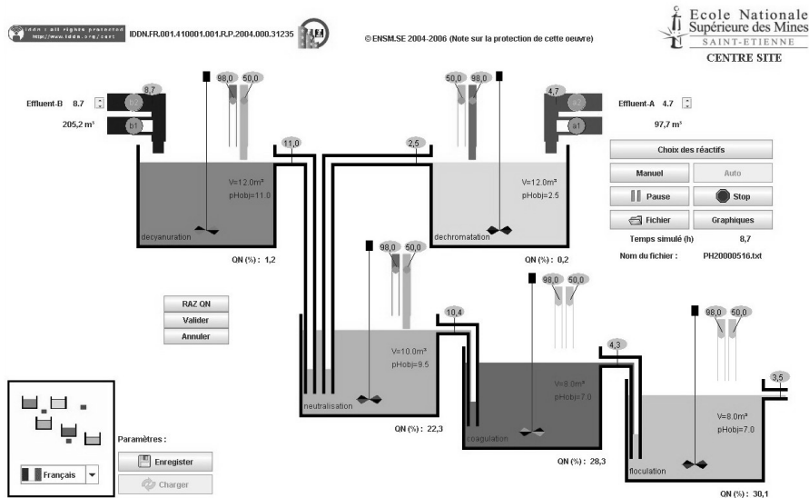
Figure 2. Multiple-CFSTR simulator main screen. The user interface is here in French; but it can be adapted and translated in real-time into other languages (English, German, Polish, Portuguese, Chinese...).
